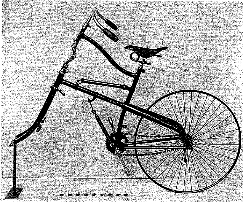
Figure 8.14 Whippet spring frame (1885). Photograph courtesy of the Trustees of the Science Museum, London.
