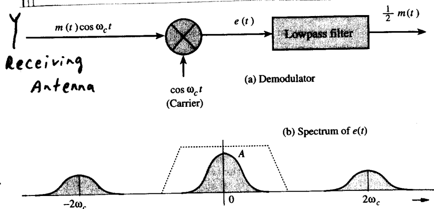
Fig. 4.33 Demodulation of DSB-SC.
