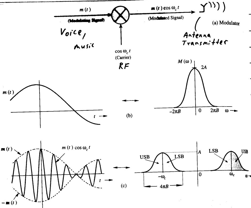
Fig. 4.31 DSB-SC modulation.
