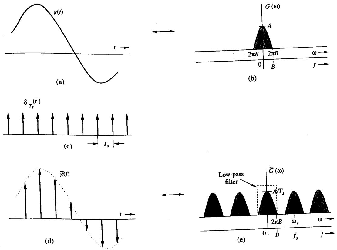
Figure 6.1 Sampled signal and its Fourier spectrum.
