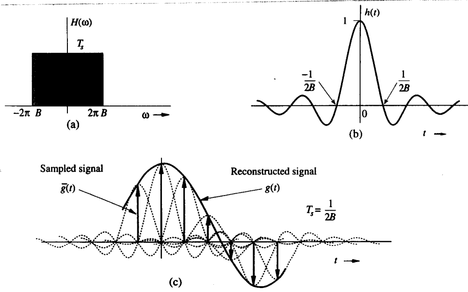
Figure 6.3 Ideal interpolation.
