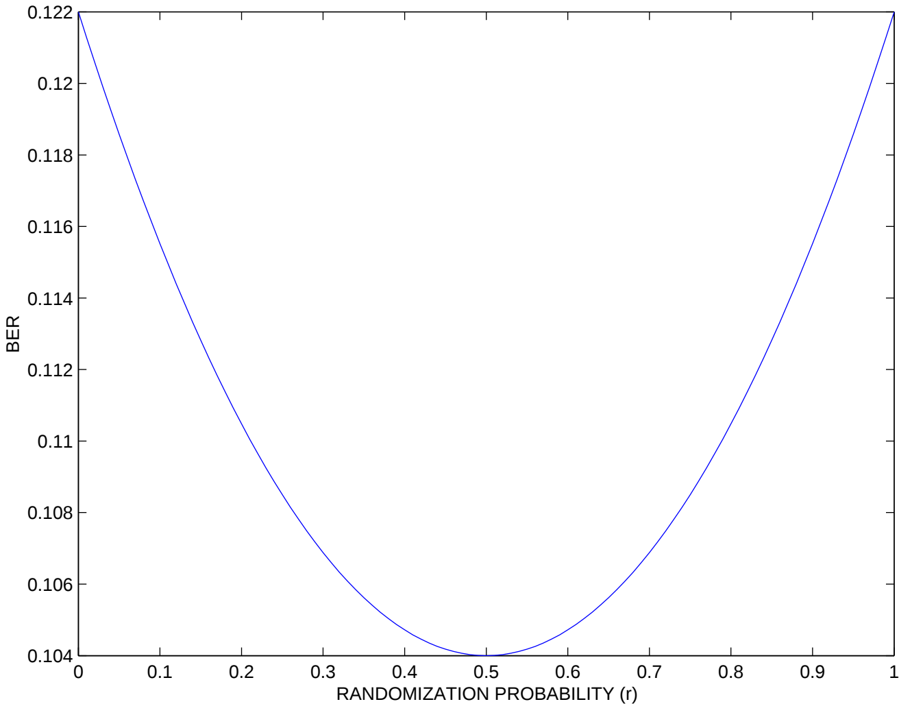
BER FOR 3 TIMES REPETITION AND MAJORITY
