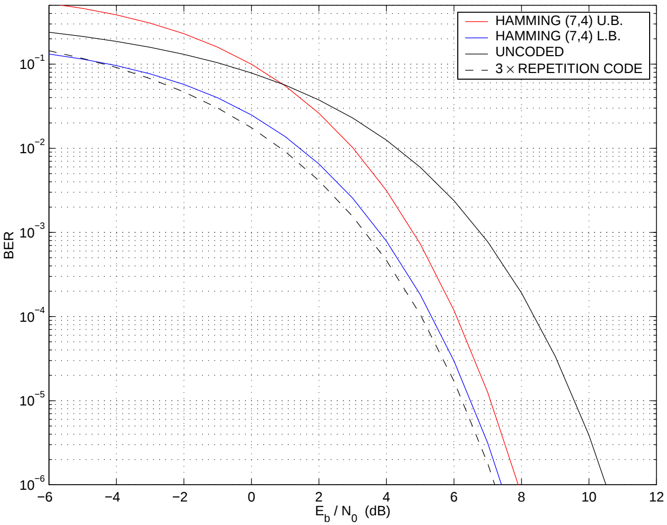
BER FOR BPSK IN AWGN
