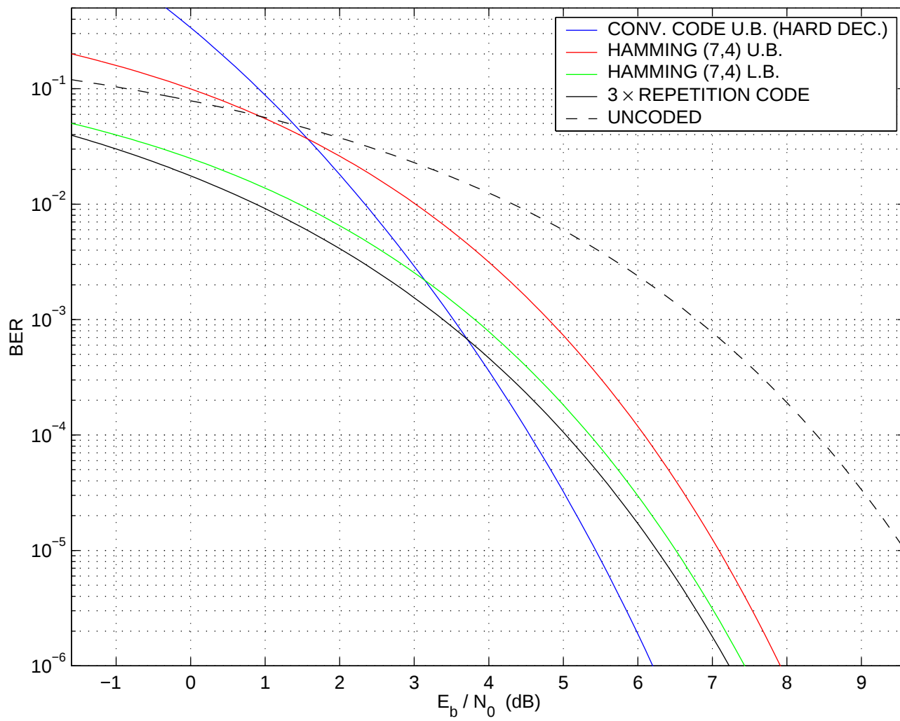
BER FOR BPSK IN AWGN
