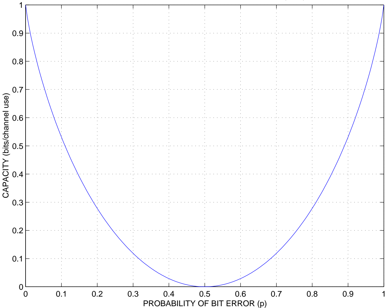
CAPACITY OF BINARY SYMMETRIC CHANNEL (BSC)
