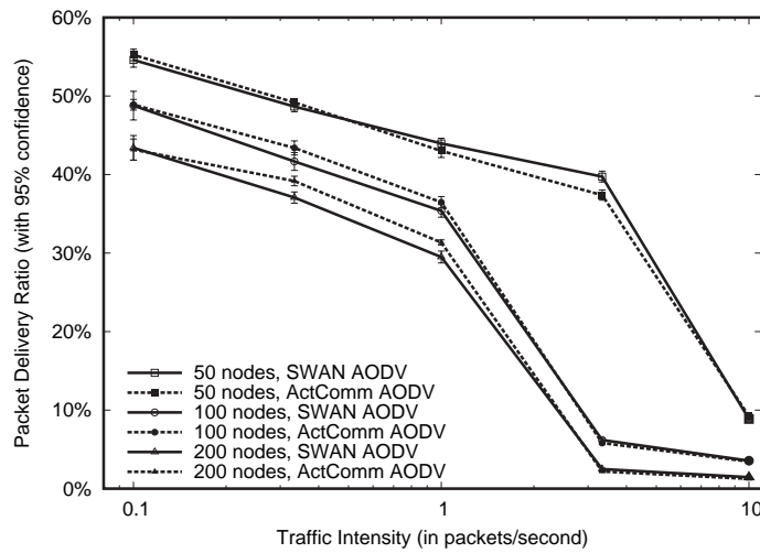
Figure 3. Packet delivery ratio with varying traffic load (in log scale)
