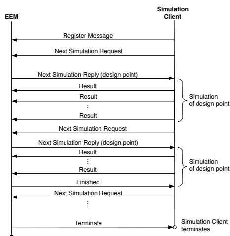
Figure 2: Communication protocol for EEM and SCs.
