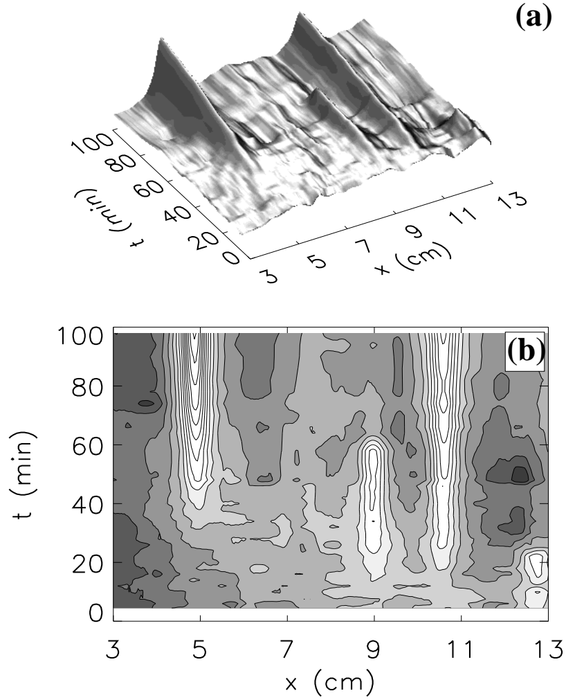
FIGURE 6. Spacetime plots of 5°C isotherm (second from bottom in Figure 4 and inside the mushy layer); 10 mm cell thickness, T_o = 10.0^\circ\text{C} . (a) Surface plot; (b) Contour plot. Bumps in the isotherms – indicating upward flows – are revealed as elevations in the surface plot (a) and as bright regions in the contour plot (b). The plumes that develop at the far left and far right (see Figure 4) of the cell are not included in these plots.
