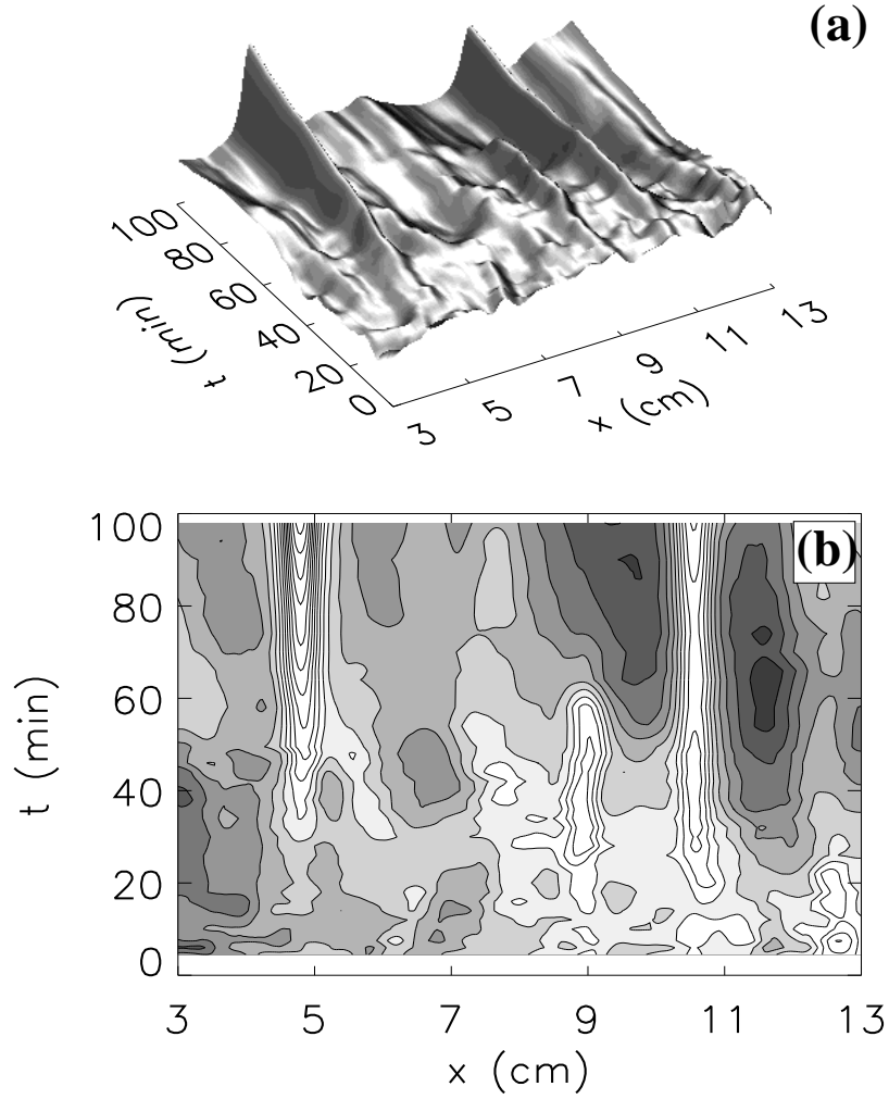
FIGURE 7. Spacetime plots of 9^{\circ}\text{C} isotherm (third from bottom in Figure 4, in the liquid region above the mush); 10 mm cell thickness, T_o = 10.0^{\circ}\text{C} . (a) Surface plot; (b) Contour plot.
