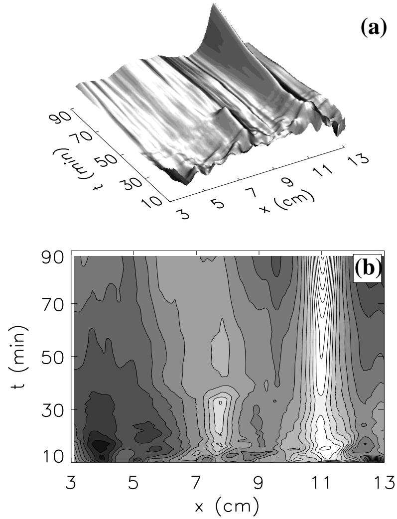
FIGURE 10. Spacetime plots of evolution of 5°C isotherm (second from bottom, inside the mushy layer) for run shown in Figure 9; 2.0 mm thickness, T_o = 10.0^\circ\text{C} . (a) Surface plot; (b) Contour plot.
