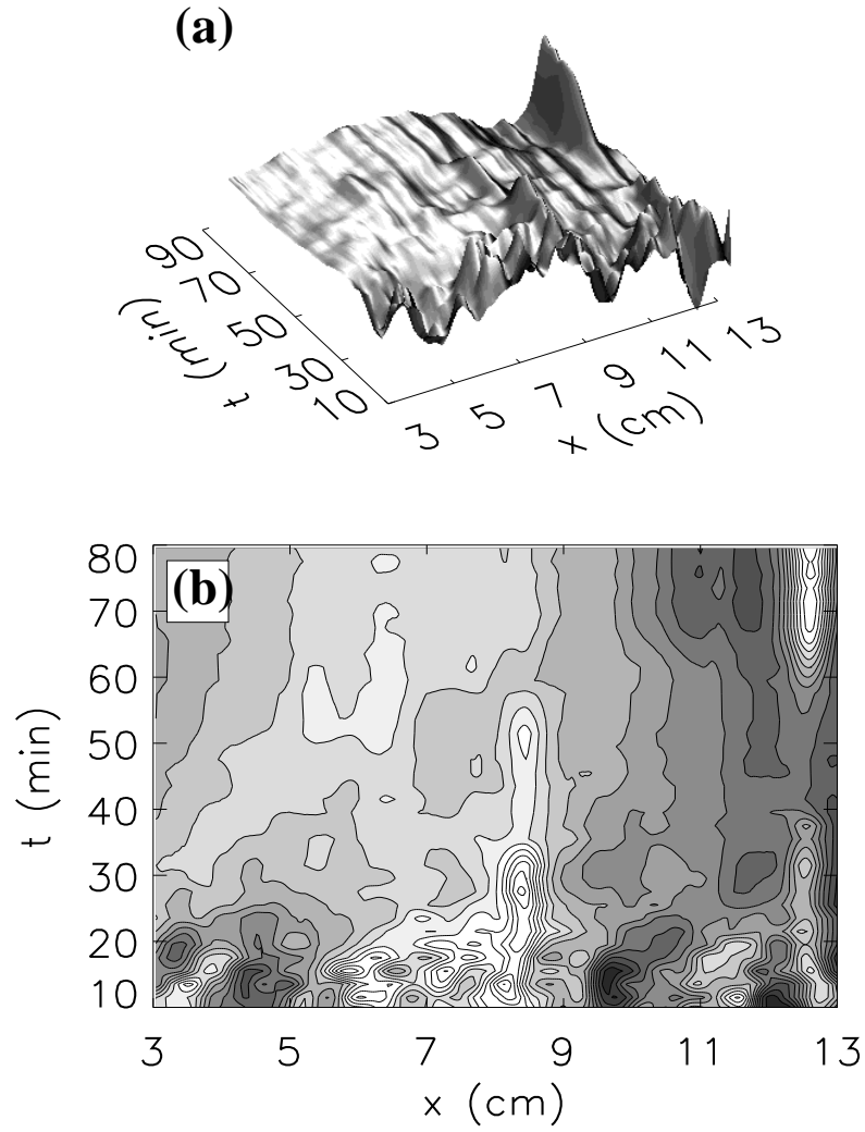
FIGURE 14. Spacetime plots of evolution of 9^{\circ}\text{C} isotherm (in the mushy layer) for run shown in Figure 13; 2.0 mm thickness, T_o = 15.0^{\circ}\text{C} . (a) Surface plot; (b) Contour plot. Oscillations can be observed in the plume intensities, with plumes at x = 8.5 cm and x = 12.7 cm oscillating out of phase with each other.
