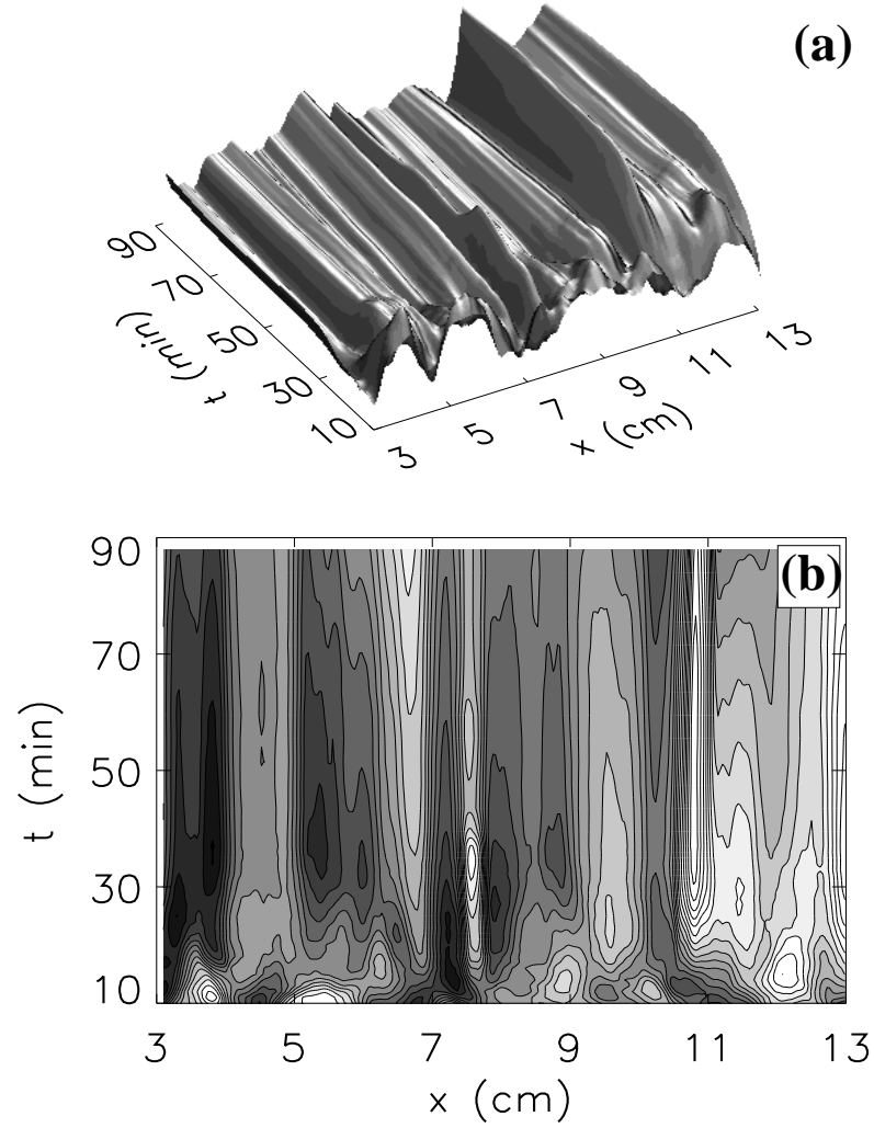
FIGURE 11. Spacetime plots of the solid fraction profile for the run shown in Figure 9; 2.0 mm thickness, T_o = 10.0^\circ\text{C} . High points in these plots represent regions of low solid fraction; a large peak therefore represents a chimney. Chimneys initially form at x=7.7 and 10.9 cm. (a) Surface plot; (b) Contour plot.
