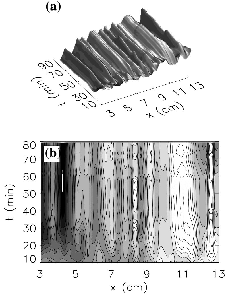
FIGURE 15. Spacetime plots of the solid fraction profile for the run shown in Figure 13; 2.0 mm thickness, T_o = 15.0^\circ\text{C} . High points in these plots represent regions of low solid fraction; a peak therefore represents a chimney. Chimneys form at x=8.5 and 12.7 cm and oscillate out of phase with each other. (a) Surface plot; (b) Contour plot.
