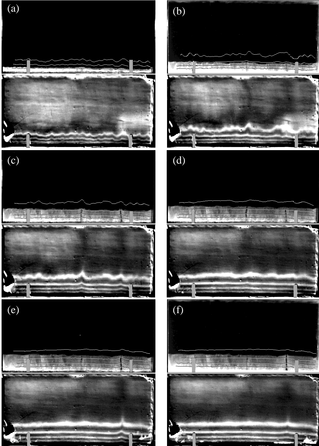
FIGURE 13. Sequence showing solidification in a 2.0 mm thick cell; T_o = 15.0^\circ C . In each frame, the top image shows the growing NH_4Cl mushy layer, and the bottom shows the corresponding TLC image. Time after start of run for images: (a) 10 min; (b) 20 min; (c) 30 min; (d) 50 min; (e) 70 min; (f) 100 min.
