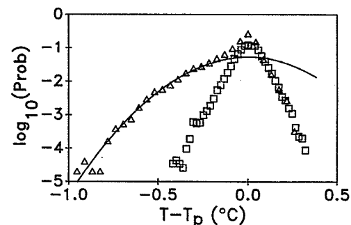
FIG. 15. Transition in the center probability distribution function (PDF) induced by single-vortex forcing at Ra=1.2 \times 10^8 . The cases shown are unperturbed ( \square ) and forced with v_f=5.7 cm/s ( \Delta ). The peak temperature T_p has been subtracted from the temperature axis. The tails of the PDF are fitted to an exponential in the unperturbed ( \square ) case and to a Gaussian in the forced ( \Delta ) case. The transition in the PDF is associated with more coherent plumes.
