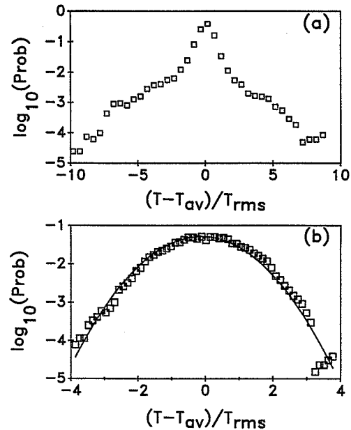
FIG. 14. Dependence of the center probability distribution function (PDF) on aspect ratio for soft turbulence. (a) Aspect ratio \Gamma=1.6 , Ra=4.9 \times 10^6 . The PDF is mixed, having Gaussian tails but exponential peaks. (b) \Gamma=0.7 , Ra=5.4 \times 10^6 . The PDF is Gaussian. The aspect ratio of the cell has been reduced in (b) by adding Plexiglass spacers to the interior of the small ( d=4.0 cm) cell.
