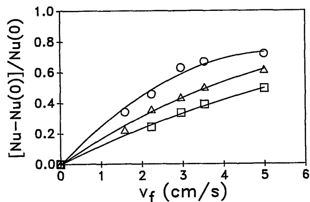
FIG. 9. Enhancement of the Nusselt number Nu by many-vortex forcing: Ra = 1.8 \times 10^7 ( \circ ), Ra = 5.0 \times 10^7 ( \triangle ), Ra = 1.0 \times 10^8 ( \square ). Curves are drawn through the data to guide the eye.
