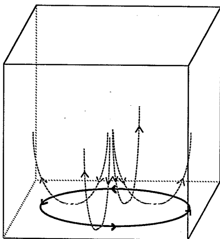
FIG. 3. Diagram of the secondary flow (dotted lines) associated with a mirror vortex (bold line). The secondary flow moves downward in the center of the vortex and upward at the edges of the vortex.
