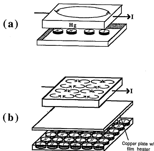
FIG. 1. Exploded view of the bottom of the convection apparatus, showing magnetohydrodynamic forcing mechanisms. (a) Single-vortex forcing. (b) Many-vortex forcing. The thin copper plate used to heat the mercury is shown in (b), but not in (a).
