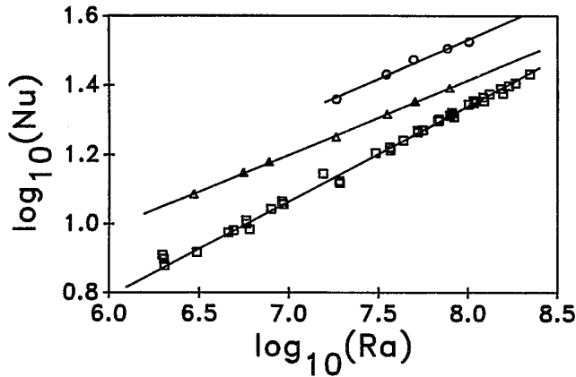
FIG. 10. Scaling of Nu with Ra , with nondimensional forcing v_f d/\kappa held constant at the following values: zero ( \square ), 9.4 \times 10^3 ( \triangle ), and 3.0 \times 10^4 ( \circ ). The heat flux is increased (and the slope reduced) by the forcing (upper two curves).
