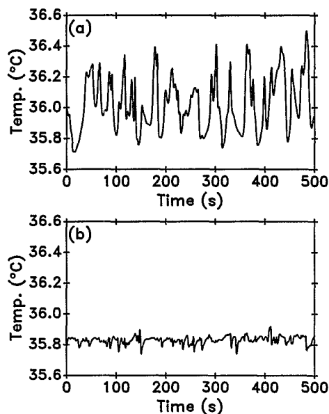
FIG. 7. Temperature time series measured at the lower probe, at Ra = 5.2 \times 10^7 . (a) Unperturbed convection. (b) Time-independent forcing by a single vortex with v_f = 3.2 cm/s. Warm temperature excursions are almost completely absent in (b), indicating a nonbursting lower boundary layer.
