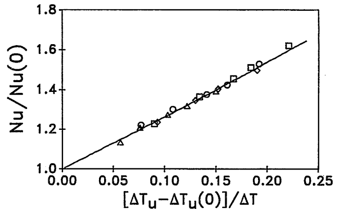
FIG. 12. The Nu enhancement (divided by the unforced Nu ) as a function of the normalized shift of the temperature drop \Delta T_u across the upper boundary layer. The symbols are the same as in Fig. 11. The solid curve is the prediction of Eq. (6). The good agreement demonstrates the independence of the two boundary layers.
