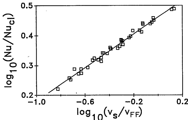
FIG. 13. Enhancement of the heat flux by external forcing as a function of the strength v_s of the induced secondary flow. The data is adjusted to correspond to the forcing of both boundary layers. The effective Rayleigh number Ra_{\text{eff}} [Eq. (7)] varies from 10^6 to 10^8 . The Nusselt number Nu is scaled by the classical prediction [Eq. (2)], and v_s is scaled by the free-fall velocity v_{\text{FF}} [Eq. (4)]. The data collapse onto a single curve with slope 0.28 \pm 0.01 .
