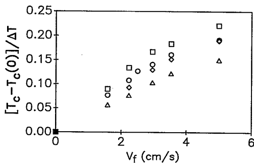
FIG. 11. Shift of the mean center temperature T_c from the unperturbed value T_c(0) as a function of the forcing velocity v_f : Ra = 3.0 \times 10^6 ( \circ ), Ra = 7.8 \times 10^6 ( \triangle ), Ra = 5.0 \times 10^7 ( \square ), Ra = 1.0 \times 10^8 ( \diamond ). The shift in T_c is scaled by the total temperature difference \Delta T .
