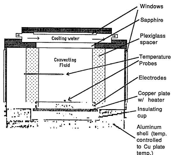
FIG. 4. Diagram of the convection apparatus. The gap between the plexiglass spacer and the outer shell is filled with styrofoam when quantitative measurements are made.
