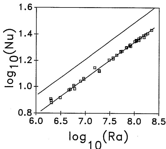
FIG. 5. Scaling of the Nusselt number Nu with Rayleigh number Ra for unforced convection, along with a power-law fit [Eq. (3)]. The top curve is the experimental result of Chu and Goldstein.
