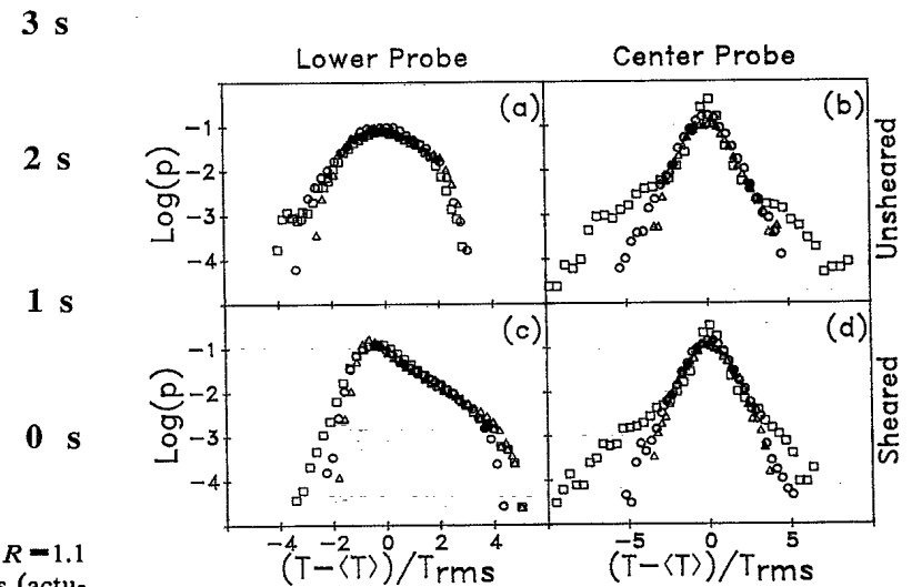
FIG. 5. Temperature probability distribution functions: R=4.9 \times 10^6 ( \square ), 5.7 \times 10^7 ( \Delta ), 1.1 \times 10^8 ( \circ ). The data are scaled by subtracting the mean temperature \langle T \rangle and dividing by the rms temperature fluctuations T_{rms} . (a) Unsheared, lower probe; (b) unsheared, center probe; (c) sheared (6 mm/s), lower probe; (d) sheared, center probe.
