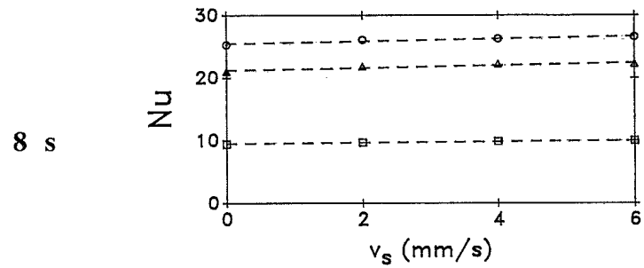
FIG. 4. Dependence of heat flux on rms forcing velocity v_s : R=4.6 \times 10^6 ( \square ), 5.7 \times 10^7 ( \Delta ), 1.1 \times 10^8 ( \circ ).
