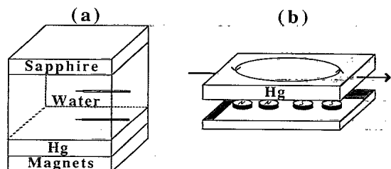
FIG. 1. (a) A schematic diagram of convection apparatus, showing temperature probes in the water layer. The sapphire window and mercury are maintained at constant temperatures. (b) Exploded view of magnetohydrodynamic forcing of a vortical flow in the mercury layer.
